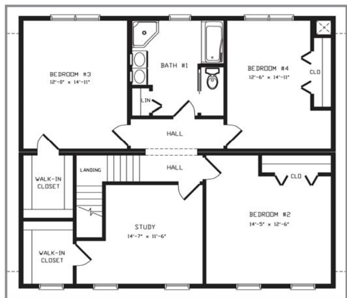
Second Story
