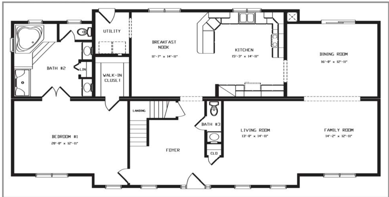
First Story
